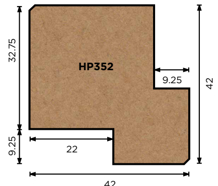
HP352 Internal Corner
