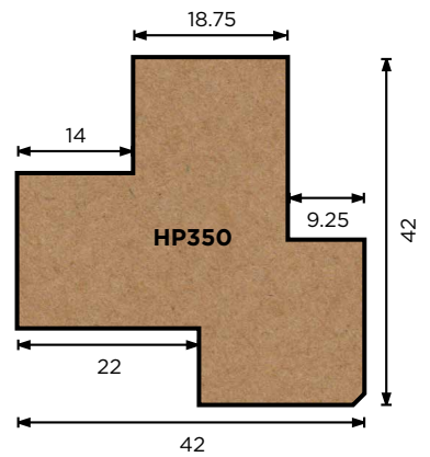
HP350 Internal Corner
