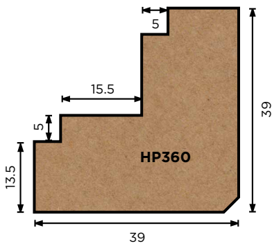
HP360 Internal Corner
