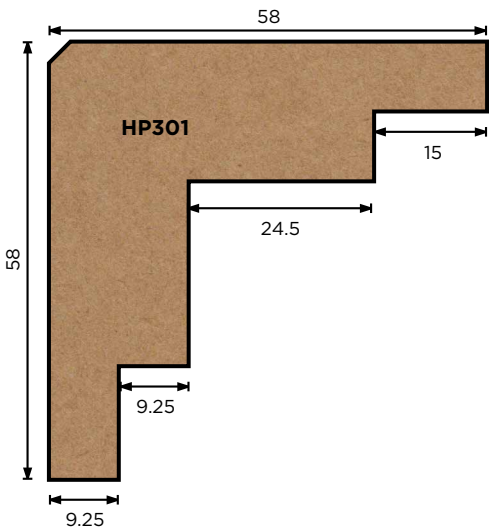
HP301 External Corner
