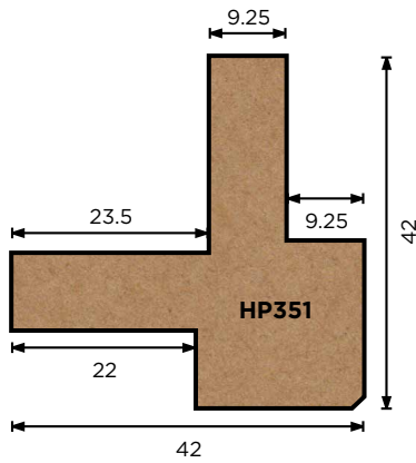
HP351 Internal Corner
