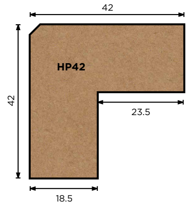
HP42 External Corner
