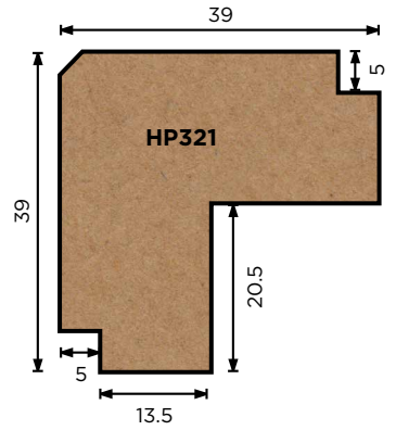
HP321 External Corner
