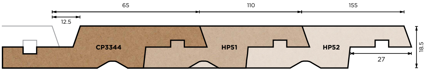
CP3344, HP51 & HP52 Vertical Shiplap
