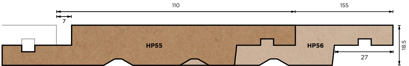
HP55 & HP56 Vertical Shiplap
