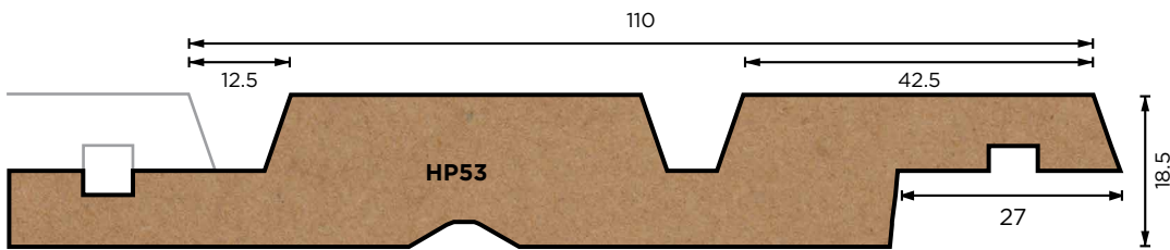
HP53 Vertical Shiplap
